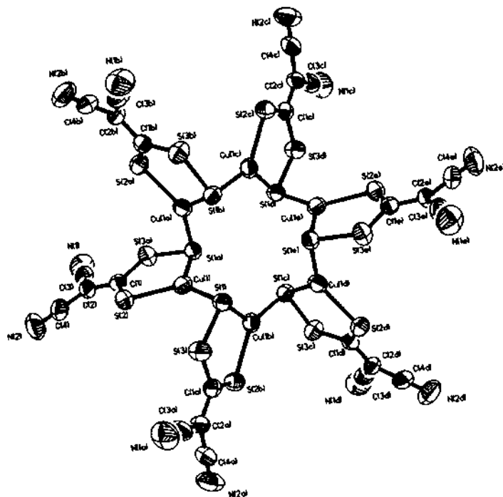
Fig. 5. Thermal ellipsoid drawing of [\text{Cu}_6(\text{S}_4i\text{-MNT})_6]^{6+} \cdot 2 (50% probability).
