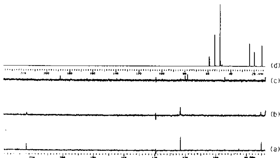
Fig. 4. The ^{13}\text{C}\{^1\text{H}\} -NMR spectra in the presence of 3 : (a) [\text{Bu}_4\text{N}]_2[\text{i-MNT}] in MeOH; (b) after adding 3 ; (c) after adding \text{CH}_2\text{Cl}_2 ; and (d) the spectra of the quaternary ammonium salt and the solvent molecules.
